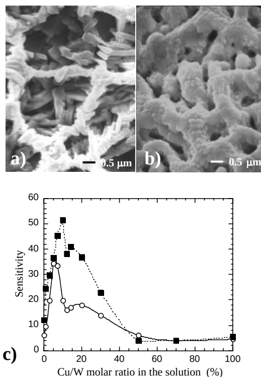
Figure 9. SEM micrograph for (a) \text{WO}_3 and (b) \text{CuWO}_{4-x} films obtained from a solution with the Cu/W molar ratio of 7%, and (c) the gas sensitivity vs molar ratio Cu/W from the solution used to obtain the films and being exposed to 5 ppm of ethanol (○) and butanol (■) in air. The operating temperature is 400 °C.
