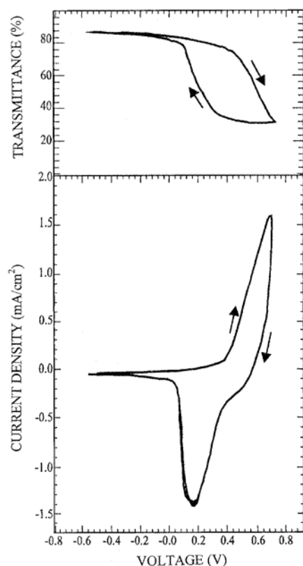
Figure 5. Cyclic voltammetric curve for a \text{NiO}_x film obtained from an alcoholic solution (bottom) and the in-situ transmittance at \lambda = 632.8 \text{ nm} (top). The scan rate was 10 mV/s and the electrolyte was aqueous 0.1 M KOH.
