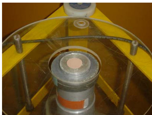
Fig. 4. Powdered samples placed in the EDXRF
