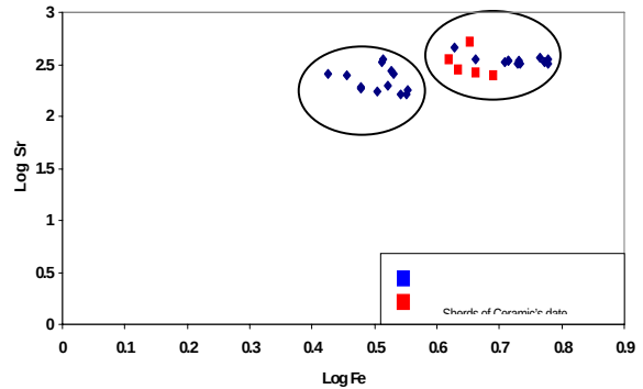
Figure 8. EDXRF composition analysis including whole vessels.
