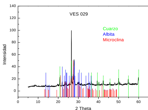
Figure 11. XRD pattern of the sample VES 029
