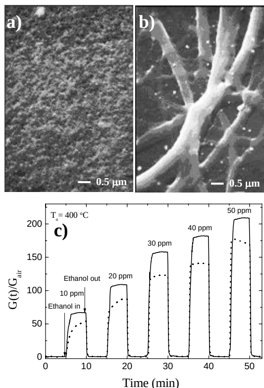
Figure 10. SEM micrographs for a nanocrystalline SnO 2 obtained from (a) an inorganic and (b) metal alkoxide precursors, and (c) their conductance response ( G(t)/G_{air} ) vs. time, to different ethanol concentrations in air. The dotted and solid line correspond for films obtained from an inorganic and metal alkoxide, respectively.
