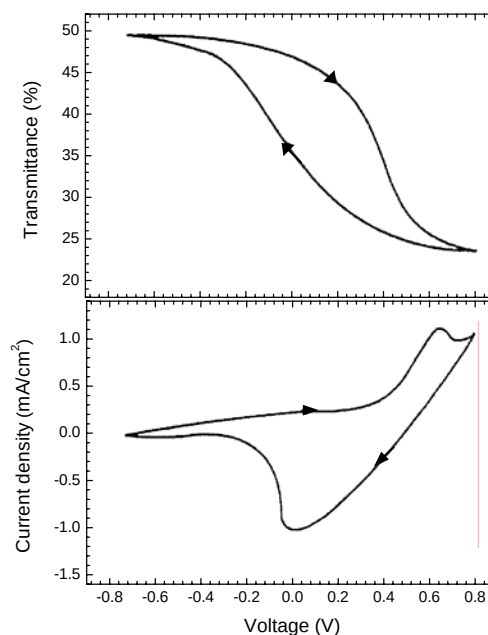
Figure 7. Cyclic voltammetric curve (bottom) and associated transmittance at 632.8 nm (top) for a pyrolytic nickel-oxide-based coating obtained from an aqueous solution of nickel nitrate. Electrolyte: 0.1 M KOH. Scan rate: 10 mV/s.
